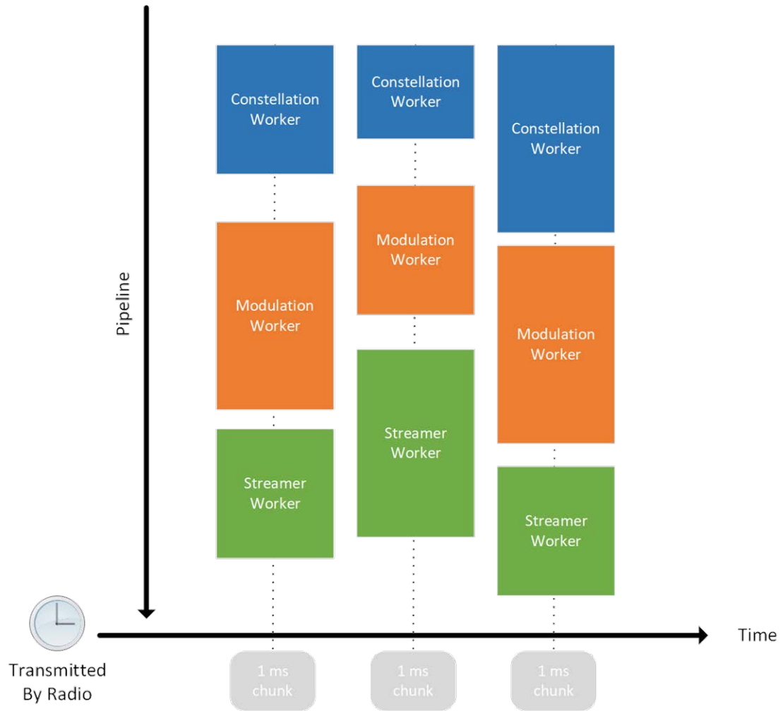
Figure 3-6: Pipeline
