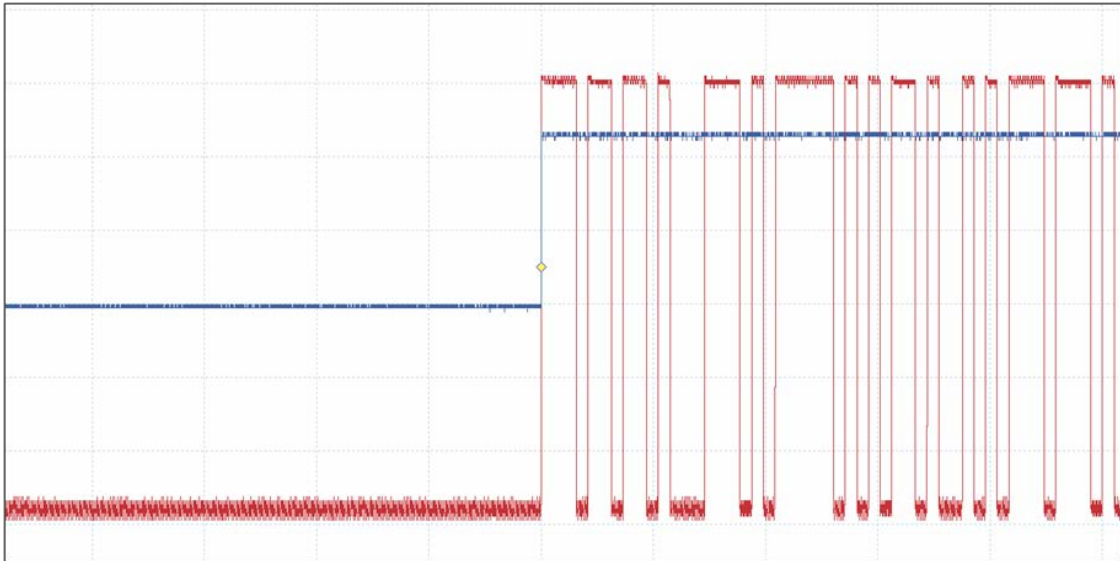
Figure 8-4: Configuration 1: Timing offset=0ms. 1PPS in blue and NMEA messages in red.
