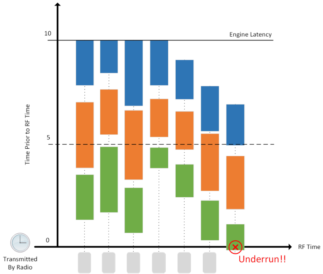
Figure 3-8: Pipeline underrun
