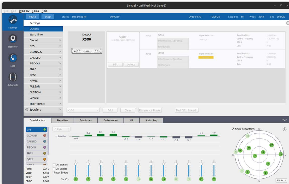
Figure 3-1: Main Window
