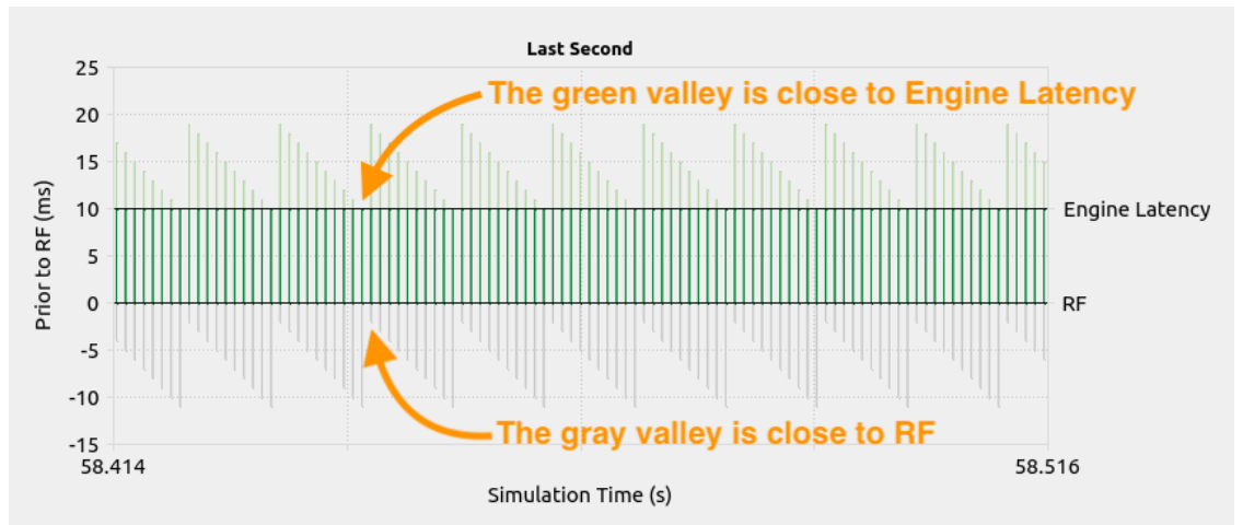
Figure 4-23: Optimal Pattern
