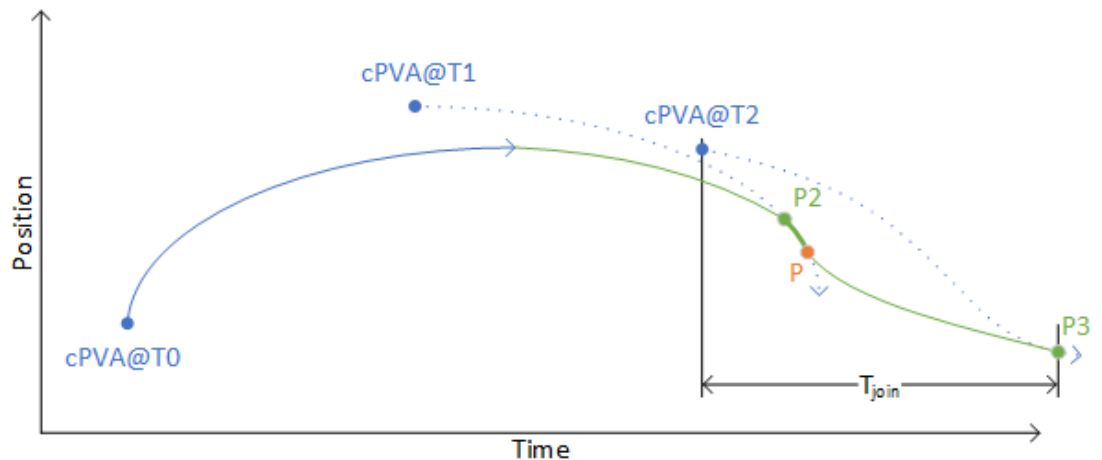
Figure 4-8: Non-Deterministic Trajectory
