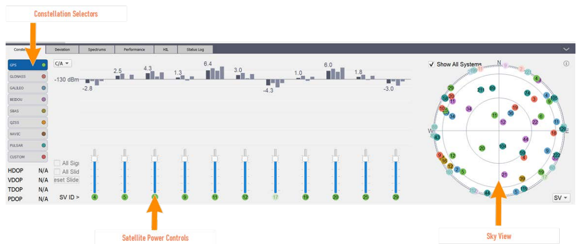
Figure 3-2: Constellations Subtab
