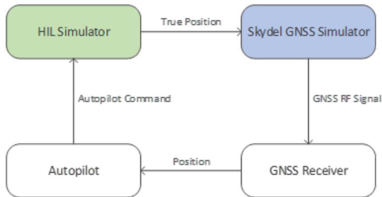
Figure 4-1: HIL Setup
