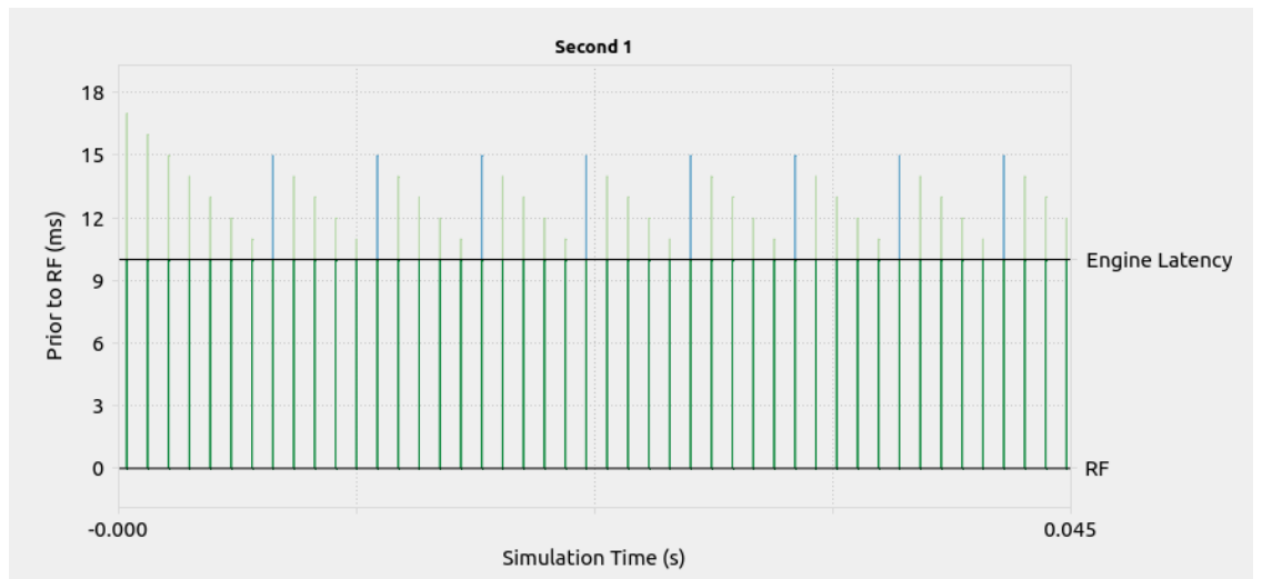
Figure 4-24: Optimal Pattern (Zoom)
