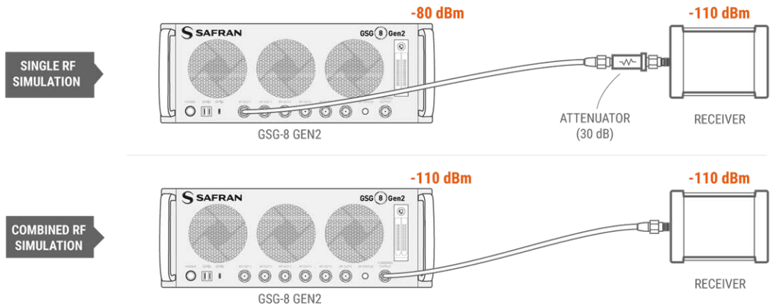
Figure 1-2: Propagation of the simulated GNSS signal from GSG-8 Gen2 to the GNSS receiver
