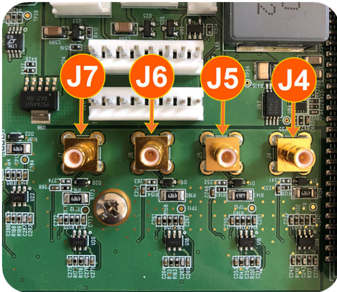
Figure 12: J Connectors (10MHz Outputs)
