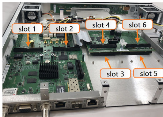
Figure 2: Unit internal view (from rear)
