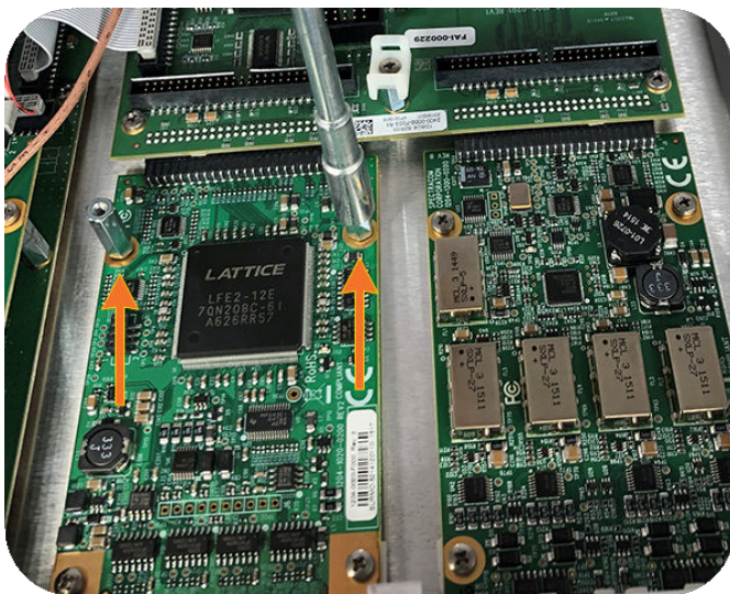
Figure 7: Bottom card with standoffs installed
