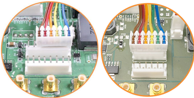
Figure 15: [Left] J19 Connector with 8 pins, [Right] J19 Connector with 6 pins, seen from rear of unit.
