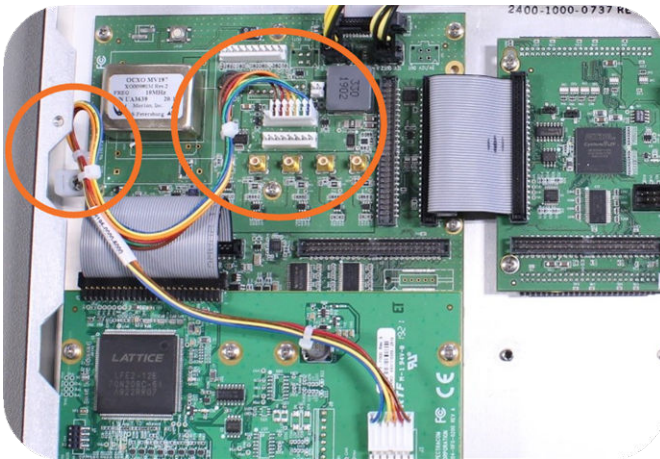
Figure 16: Cable routing
