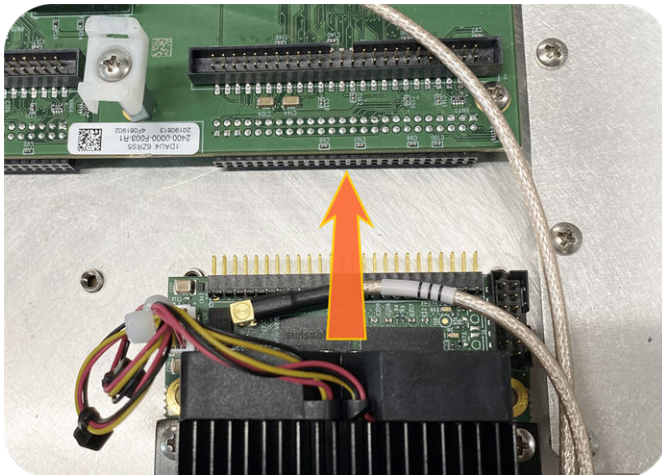
Figure 9: Connector installation
