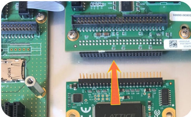
Figure 4: Connector installation
