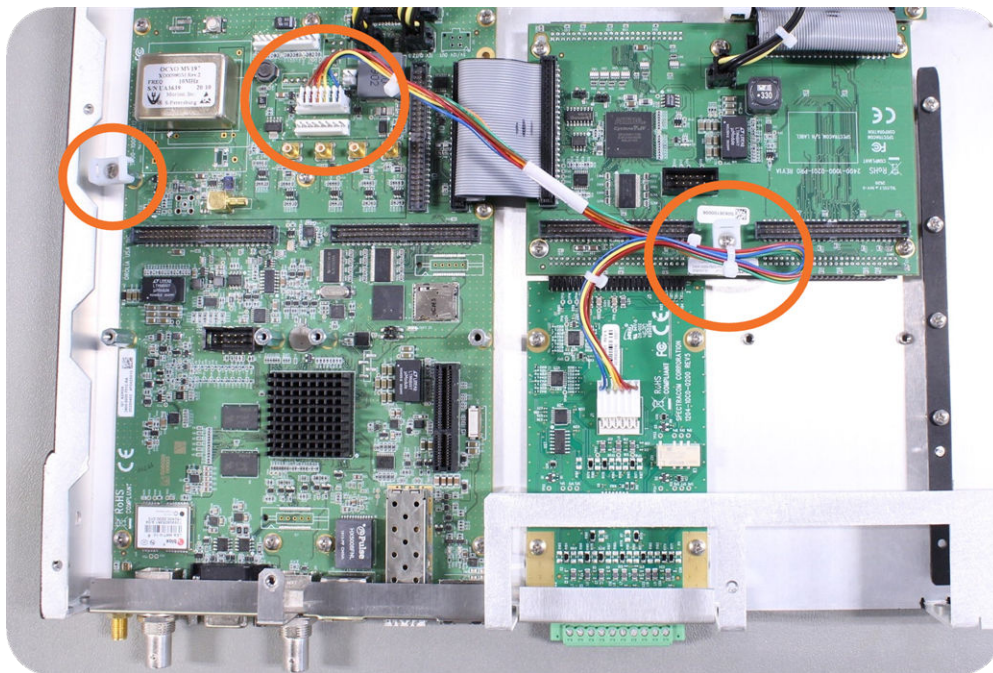
Figure 14: Cable routing
