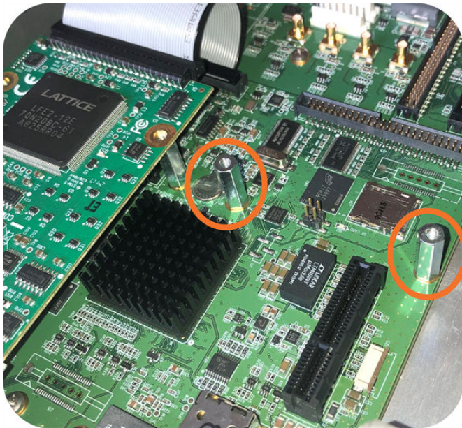
Figure 3: Standoffs location
