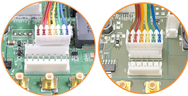
Figure 13: [Left] J19 Connector with 8 pins, [Right] J19 Connector with 6 pins, seen from rear of unit.
