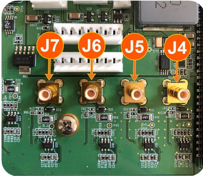
Figure 10: J Connectors (10MHz Outputs)
