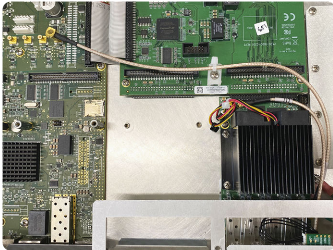
Figure 11: Completed installation
