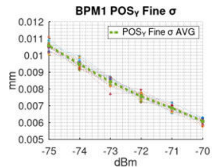
25 averaged Y position precision curves (100us integration)
