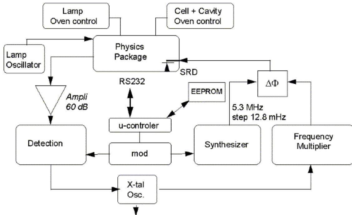
Figure 4: LPFRS block diagram
