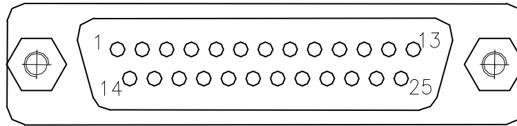
Figure 4.6-1 J2 Sub-D pin connector of LNRClOK-1500.
