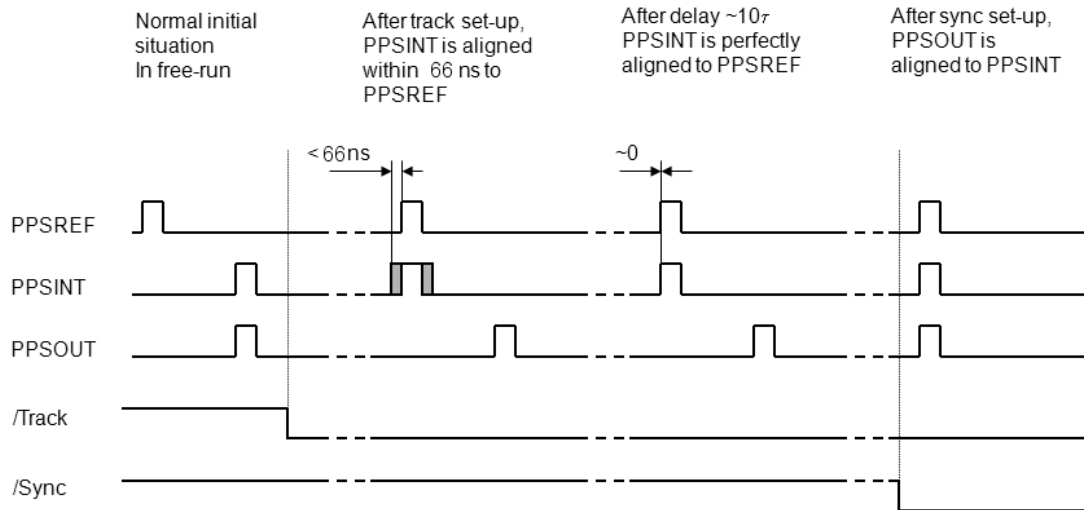
Figure 2.4-2 "Track" mode and "Sync" mode.
