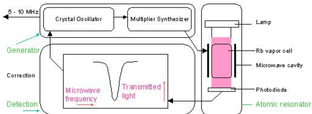
Figure 2.1-2 Rubidium atomic clock principal block diagram.
