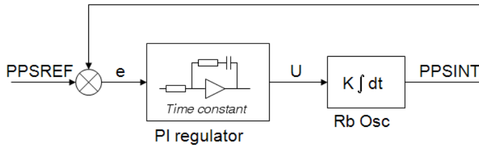
Figure 2.4-3 Schematic of the PPSREF regulation loop.
