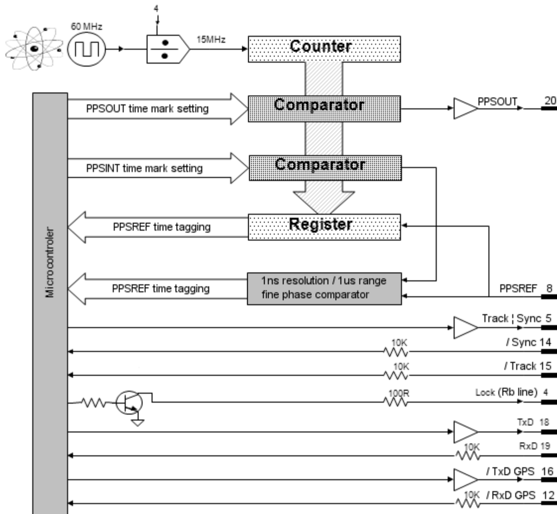
Figure 2.4-1 Timing system.
