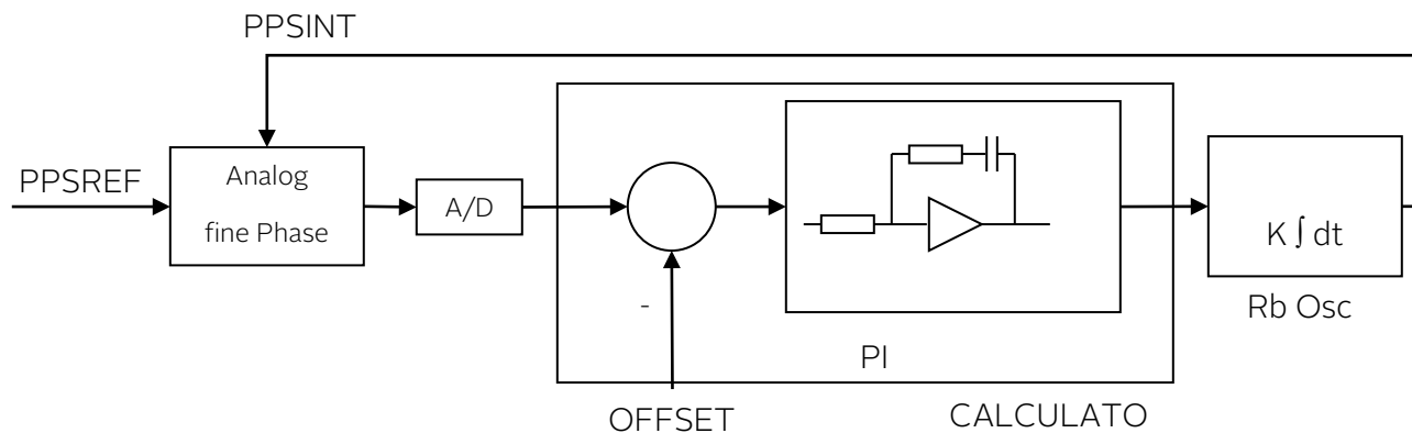
Figure 2.4-5 Schematic of the analog fine phase comparator regulation loop.
