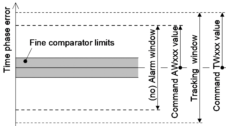
Figure 2.4-4 Tracking limits.
