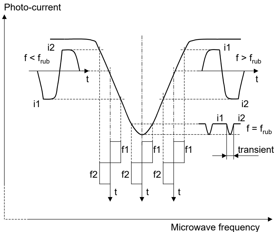
Figure 2.3-1 Dip minimum detection.
