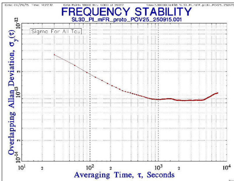
miniRAFS Typical Short Term Stability Performance
