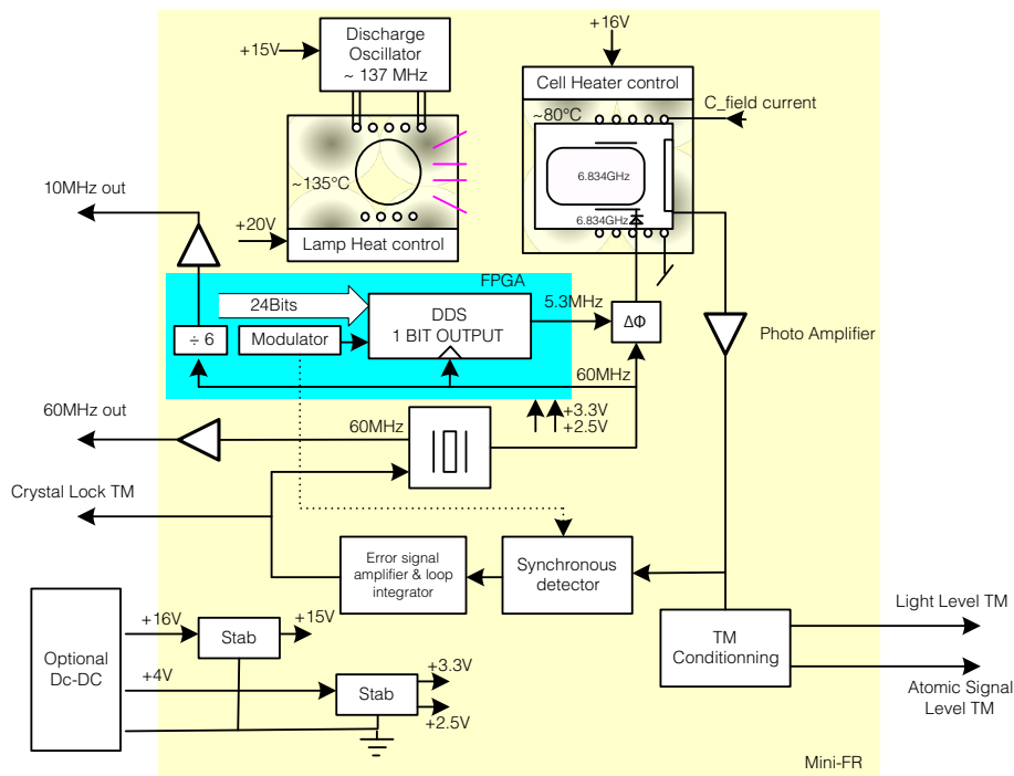
miniRAFS Functional Block Diagram
