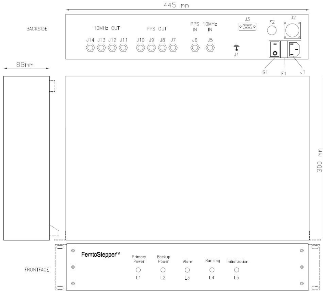
Figure 1- Mechanical Outline
