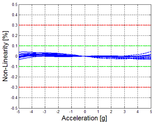
Figure 9 : Non linearity under vibration
