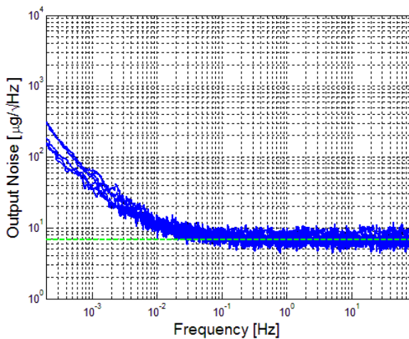
Figure 5: Typical Low Frequency Noise
