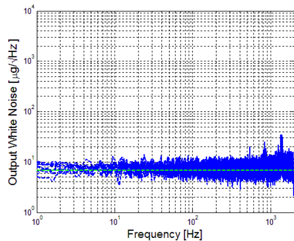
Figure 6: Typical white noise
