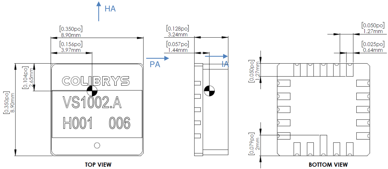
Figure 43: Package mechanical dimension
