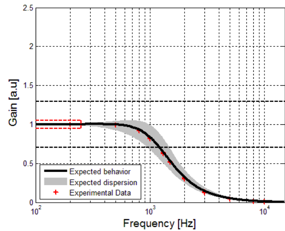
Figure 2: Typical high frequency response
