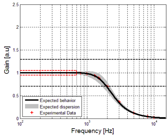
Figure 8: Typical high frequency response Courtesy of Customer
