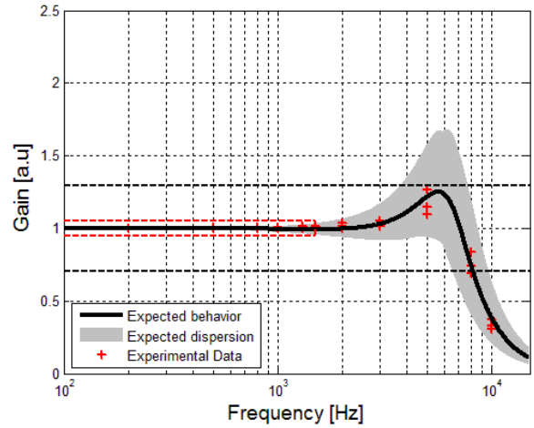
Figure 23: Typical high frequency response Courtesy of Customer
