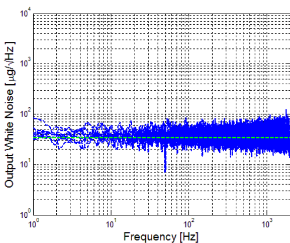
Figure 16: Typical white noise
