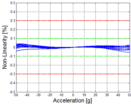
Figure 24 : Non linearity under vibration
