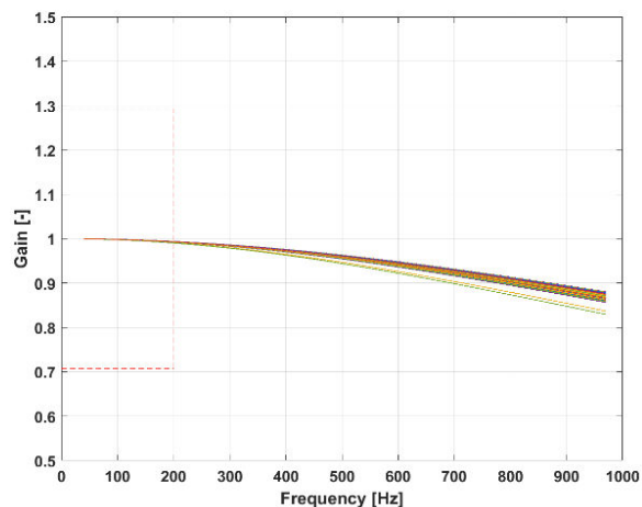
Figure 57 : Frequency response
