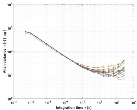
Figure 59: Allan Variance
