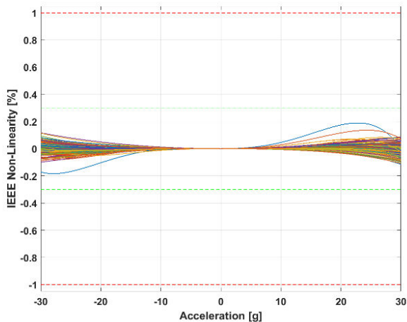
Figure 54 : Non-linearity IEEE
