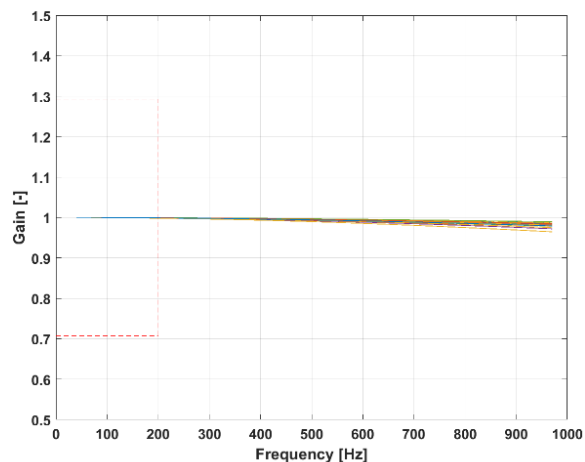
Figure 69 : Frequency response
