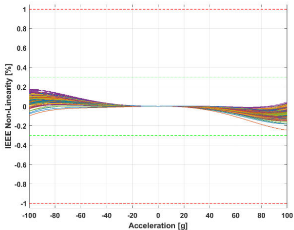
Figure 66 : Non-linearity IEEE
