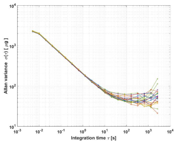
Figure 71: Allan Variance
