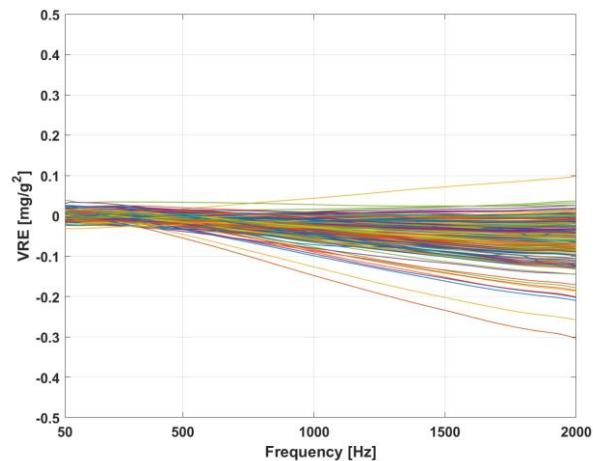
Figure 55: Vibration Rectification Error
