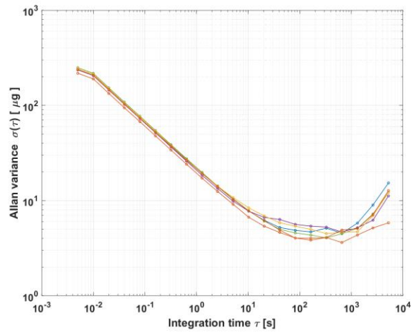
Figure 35: Allan Variance
