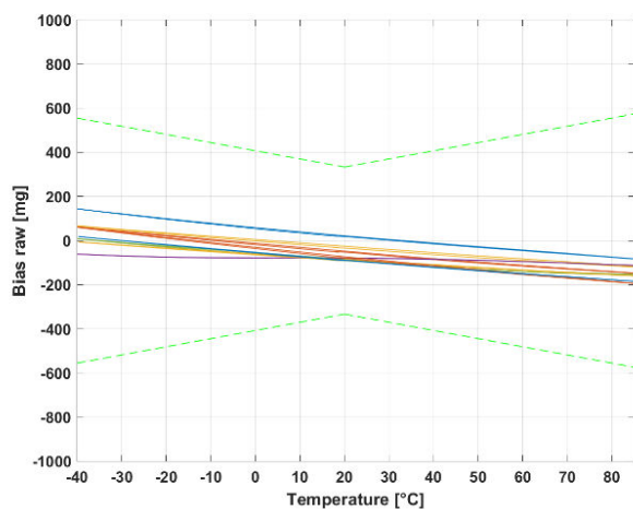
Figure 60: Raw bias over temperature
