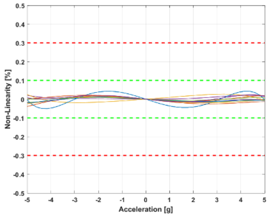
Figure 19 : Non-linearity under vibration
