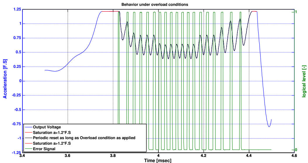
Figure 40: Overload Behavior
