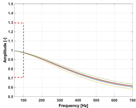
Figure 12 : Frequency response
