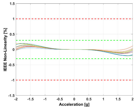
Figure 10 : Non-linearity IEEE
