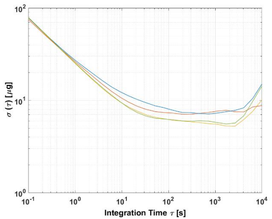
Figure 34: Allan Variance
