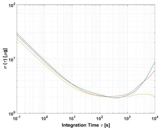
Figure 24: Allan Variance
