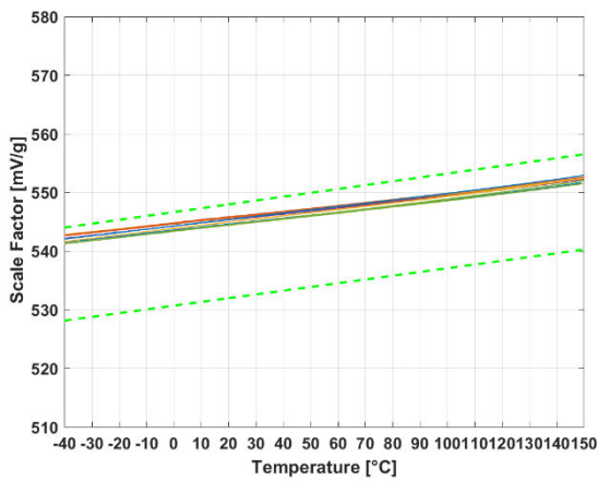
Figure 17: Raw Scale Factor over temperature
