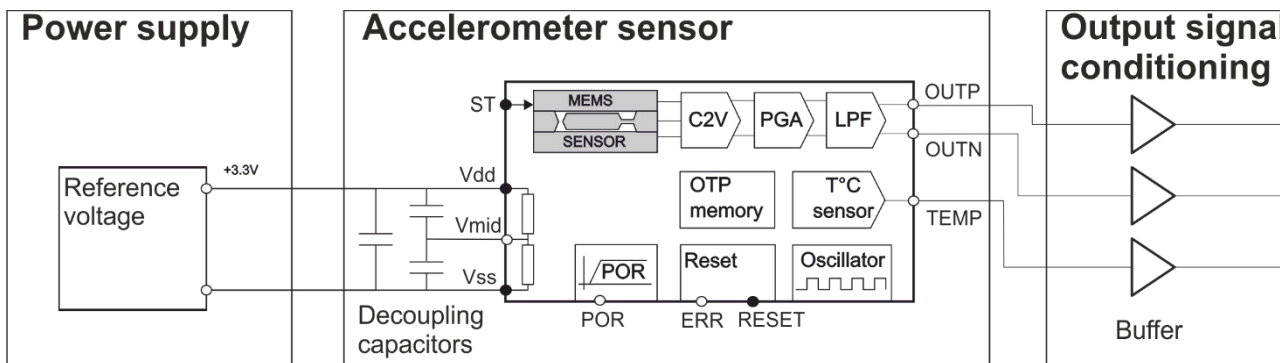
Figure 42: Block diagram
