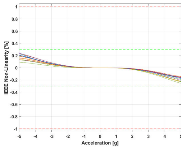
Figure 9 : Non-linearity IEEE
