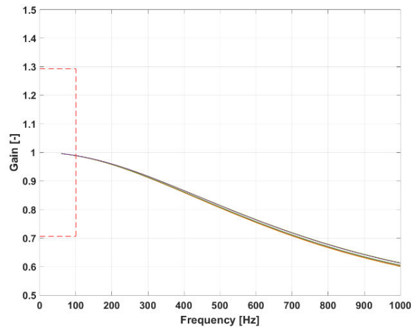
Figure 16 : Frequency response
