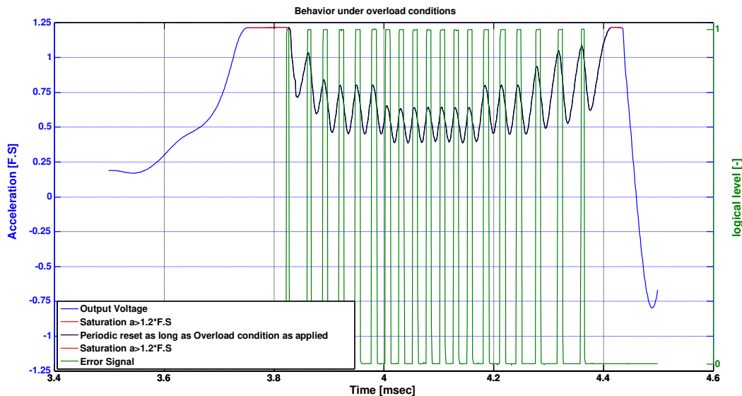
Figure 42 : Overload Behavior
