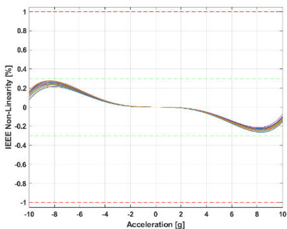
Figure 15 : Non-linearity IEEE
