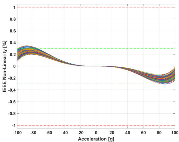
Figure 33 : Non-linearity IEEE
