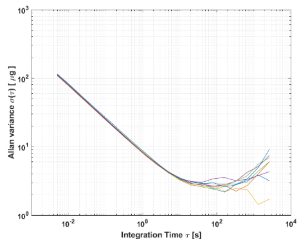
Figure 12: Allan Variance
