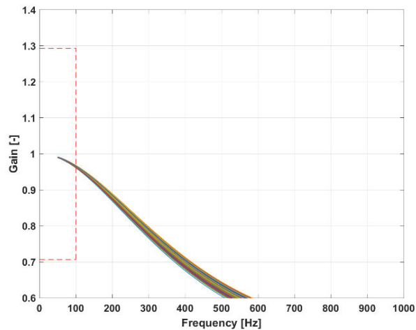
Figure 28 : Frequency response
