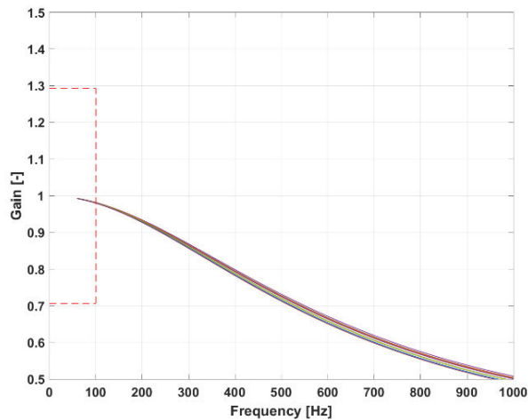
Figure 22 : Frequency response
