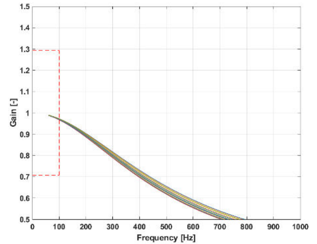
Figure 10 : Frequency response
