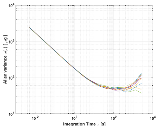
Figure 36: Allan Variance
