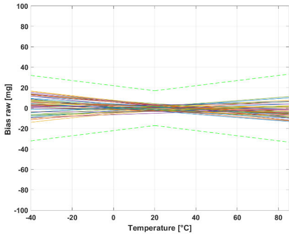
Figure 7: Raw bias
