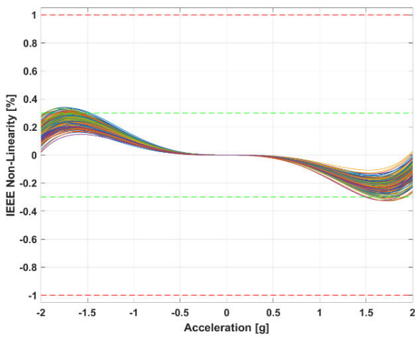
Figure 3 : Non-linearity IEEE
