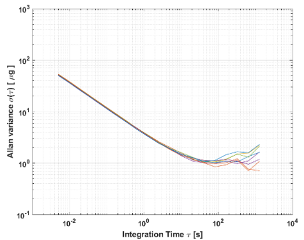
Figure 6: Allan Variance
