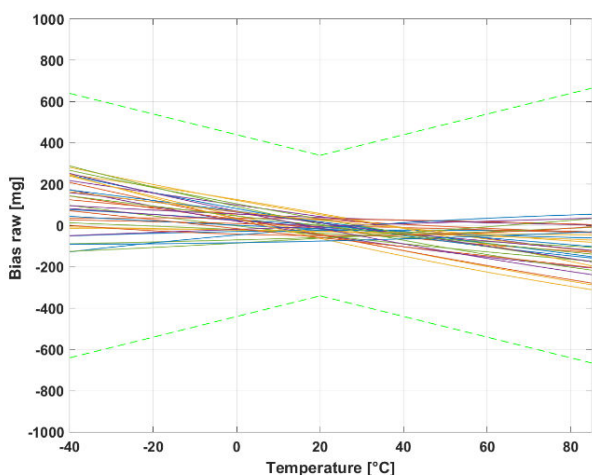
Figure 31: Raw bias
