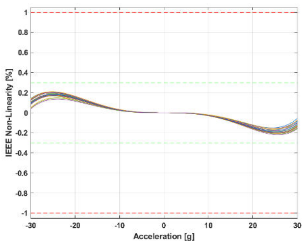
Figure 21 : Non-linearity IEEE
