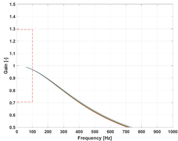
Figure 34 : Frequency response
