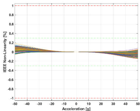
Figure 27 : Non-linearity IEEE
