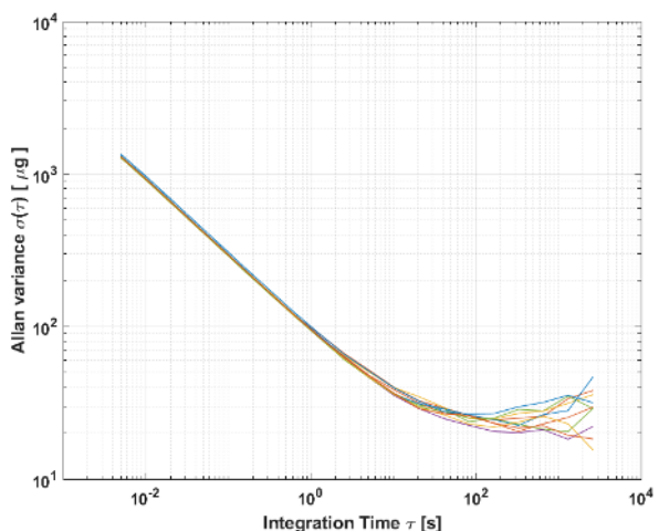
Figure 30: Allan Variance
