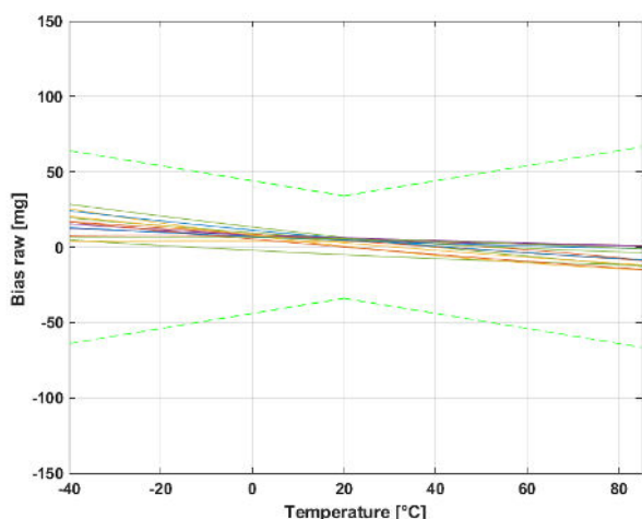
Figure 13: Raw bias
