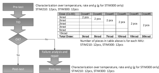
Figure 18: Total Ion Dose test flow
