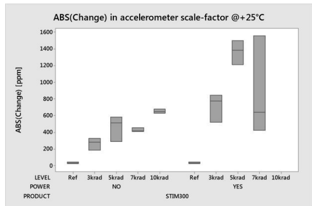
Figure 23: Change in accelerometer scale factor
